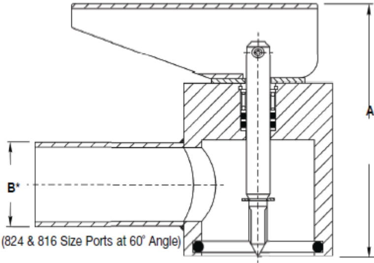
VO7 SERIES OPERATORS STAINLESS STEEL DIMENSIONS
